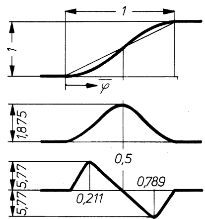
Polynom 5. Grades
