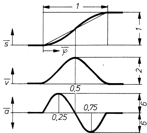
Polynom 4. Grades
